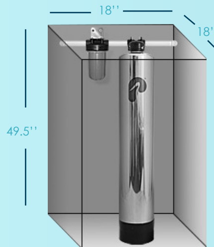
SYSTEM DIMENSIONS: PC600
